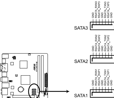
AT37N7A-I SATA connectors
